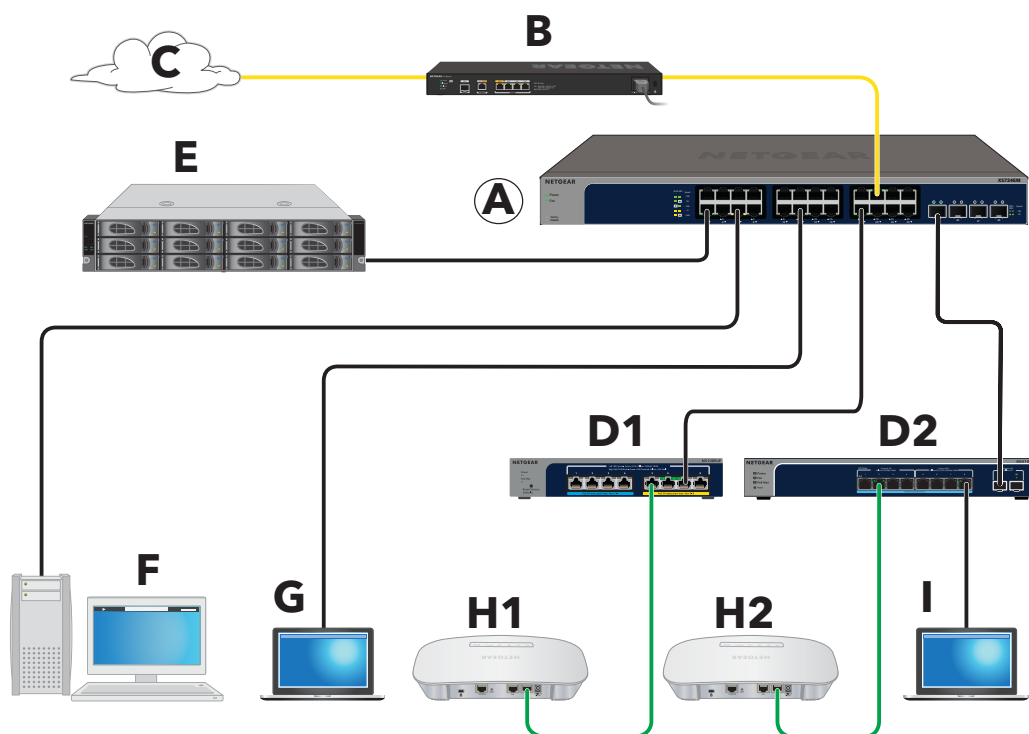
Figure 6. Sample connections
