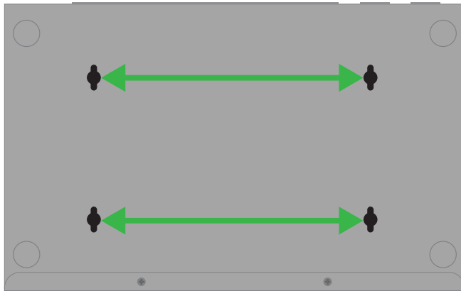
Figure 9. VESA holes at the bottom panel
