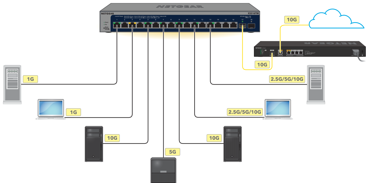
Figure 7. Sample high-speed network environment use case
