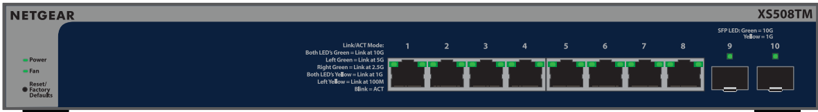
Figure 1. Front panel model XS508TM
