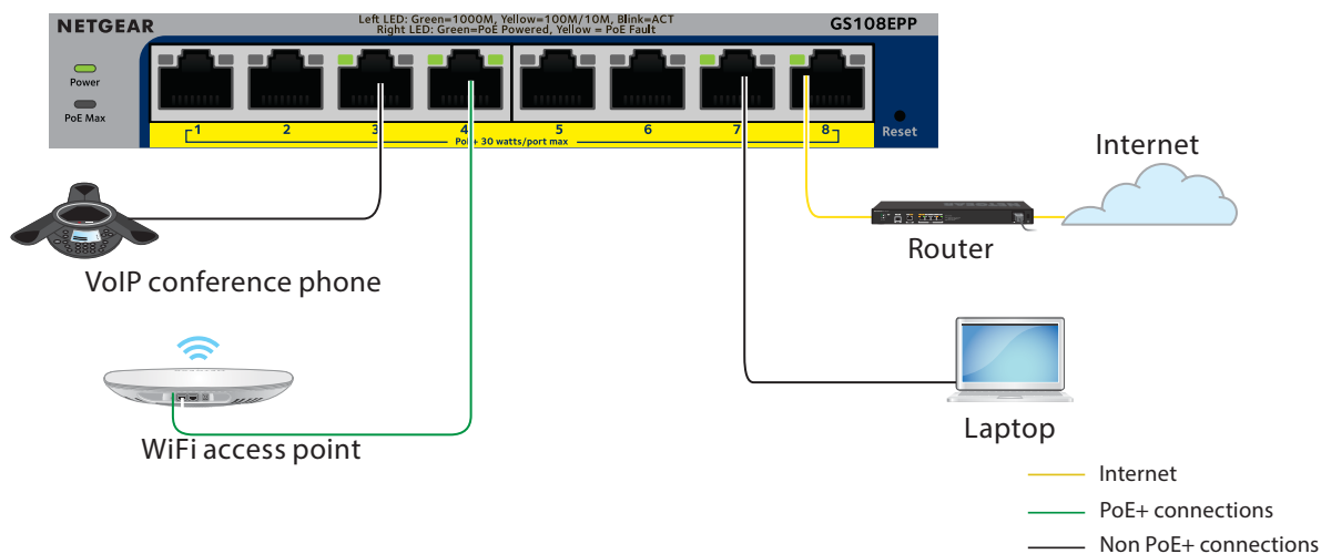
Figure 5. Example connections
