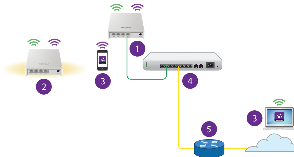
Figure 7. Mesh network with a node and a wired root
