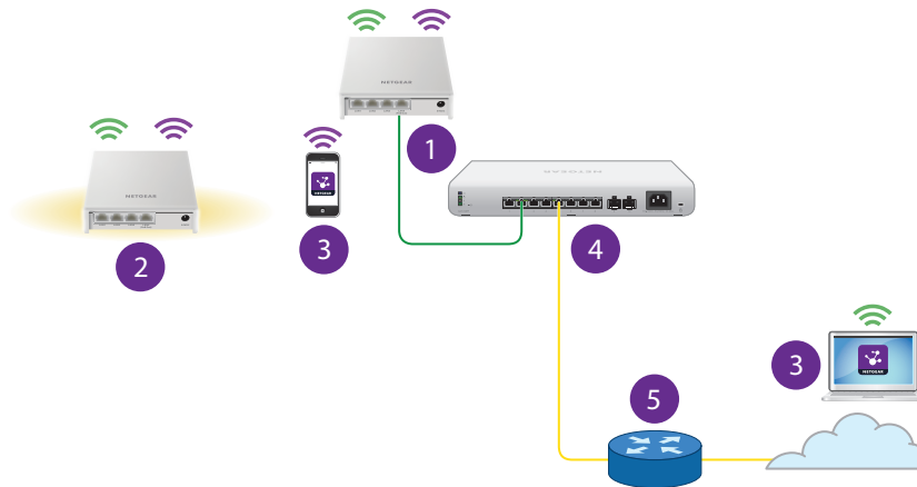
Figure 8. Connect the node to a wired root
