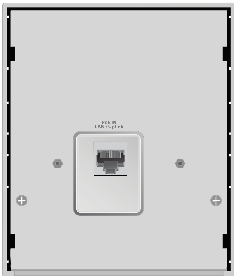
Figure 3. WAX610W back panel
